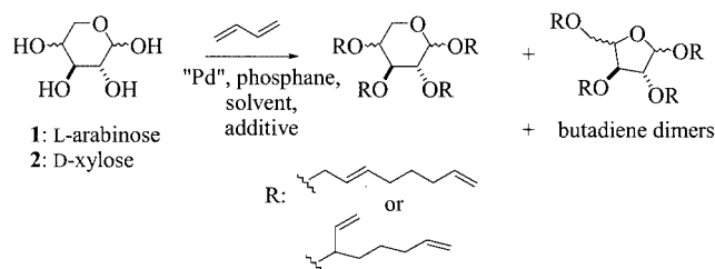
Scheme 1. Telomerization reaction of butadiene with L-arabinose and D-xylose
