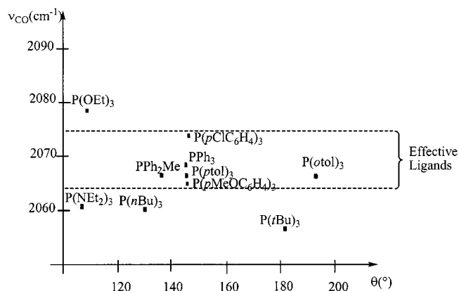
Figure 2. Steric and electronic map of the phosphanes; the \nu_{\text{CO}} values stem from IR studies of [\text{Ni}(\text{CO})_3\text{PR}_3] complexes by Tolman [31] and \theta correspond to the cone angles of the phosphane [31,32]
