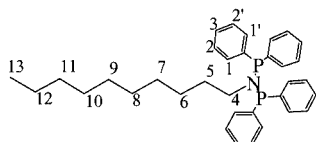
N,N -bis(diphenylphosphanyl)decylamine
