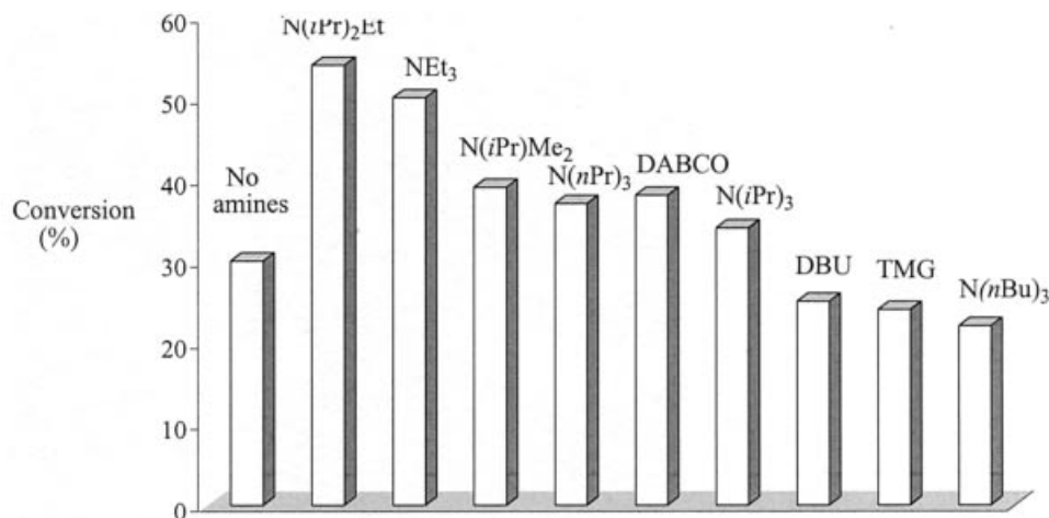
Figure 1. Effect of tertiary amines on the arabinose conversion in butadiene telomerization; conditions: Pd(acac) 2 4.4 \times 10^{-5} mol; molar ratio: L-arabinose/Pd/PPh 3 /butadiene/amine = 150:1:3:900:20; temperature 75 °C; time 140 min, 1 g of L-arabinose in 25 mL DMF
